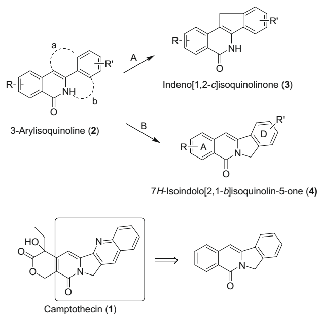
Figure 1. Structure of CPT 1 and constrained form of 3-arylisquinoline to isoindolo[2,1- b ]isoquinolin-5-one 4 .
